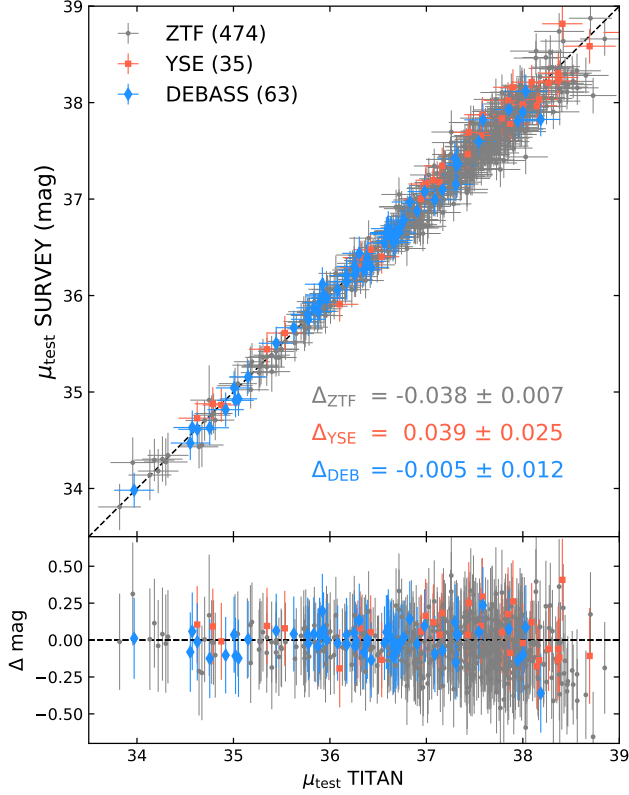
Figure 12. Fiducial distance moduli \mu_{\text{test}} for SNe Ia included in both TITAN DR1 and other modern low- z surveys. TITAN light curves are presented in the companion paper Murakami et al. (2026). Compared against ZTF DR2, DEBASS DR1, and YSE DR1. We use a conservative color error cut in TITAN SALT3 color, \sigma_c \leq 0.1 , to minimize the known error-dependent bias (see Murakami et al. 2026 for discussion). The measured offsets are consistent with zero for YSE and DEBASS. The significant offset between ZTF and TITAN is consistent with the known offset for ZTF reported in Newman et al. (2025).
