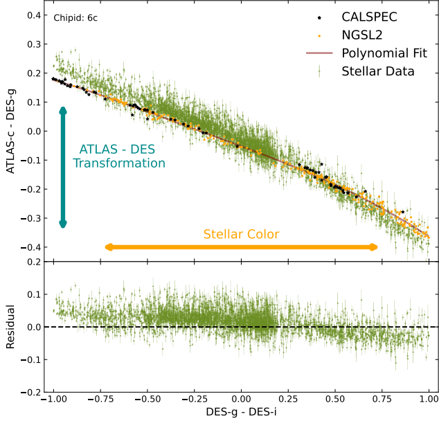
Figure 5. ATLAS - DES transformation (ATLAS-c - DES-g) versus DES color ( g - i ) for ATLAS chip 6c. Real stellar data from ATLAS server and DES Y6 is shown in green. Both NGSL and HST CALSPEC synthetic stellar photometry (orange, black) are overplotted. A 5th order polynomial is fit to the synthetic NGSL data (brown) is shown. Lower plot is the real data residual to the polynomial fit. The lower residual plot demonstrates a residual chromatic slope that must be accounted for. The net vertical shift of the green points relative to the trend line shows the inter-chip offset. The actual calculation of these offsets are substantially more complex than what is shown here and the likelihood and fitting process are described in detail in App. A. This inter-chip correction is applied after accounting for intra-chip variation.
