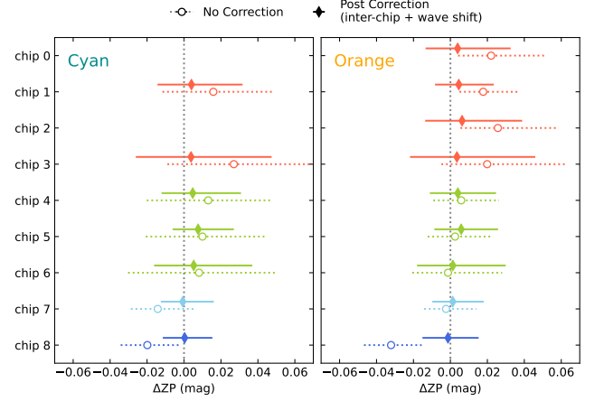
Figure 9. \Delta zeropoint offset in magnitude between observed and synthetic photometry (same definition as Fig. 8) for a validation sample of stars which are independent of Refcat2, before and after our calibration correction. The \Delta ZP value is the offset between chips and is corrected by the inter-chip correction. The error on the values is the result of a projection of the residuals from Fig. 5 into the \Delta ZP offset space, representing the scatter in residual. This error is dominated by the chromatic slope displayed in Fig. 6.
