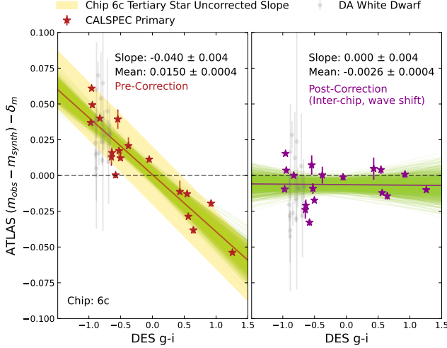
Figure 10. Synthetic minus observed residuals of several CALSPEC stars, including C26202, and DAWD, for ATLAS cyan band (chip 6c) versus DES color in g-i . This is nearly identical to the bottom panel of Fig. 5 but now demonstrating the impact of our calibration corrections. The many green lines represent random slope draws from the likelihood fit that account for covariance to show a range of possible fitted slopes and uncertainty. The solid lines are the best-fit slopes. We note that values for all chips are reported in Tab. 3
